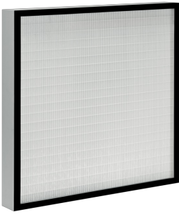
MINI PLEAT FILTER PANELS, TYPE MFP, CONSTRUCTION ALZ
