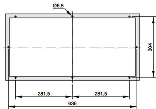
Dimensions [mm] and weight [kg] Wall mounted particulate filter with ventilation grille X-GRILLE modular
