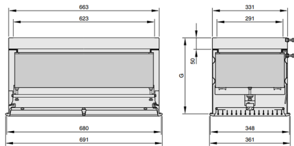
TFW flange dimensions
